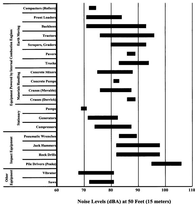
Construction Equipment Sound Levels
